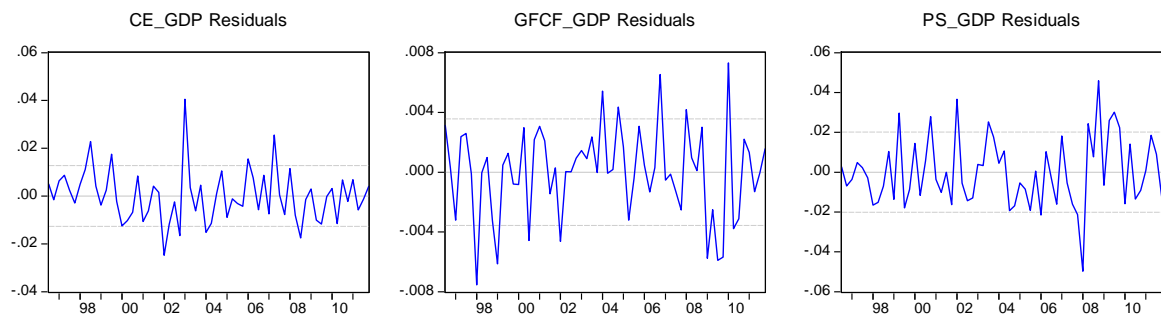
Figure A.4: Residual Graphs
