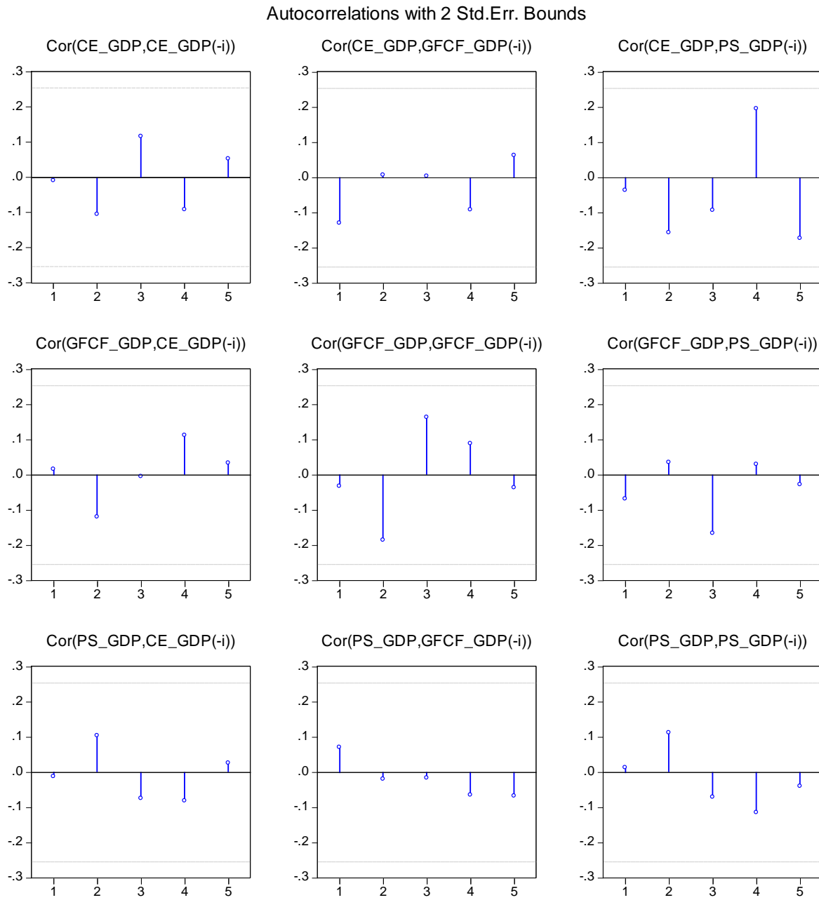
Figure A.2: Correlograms
