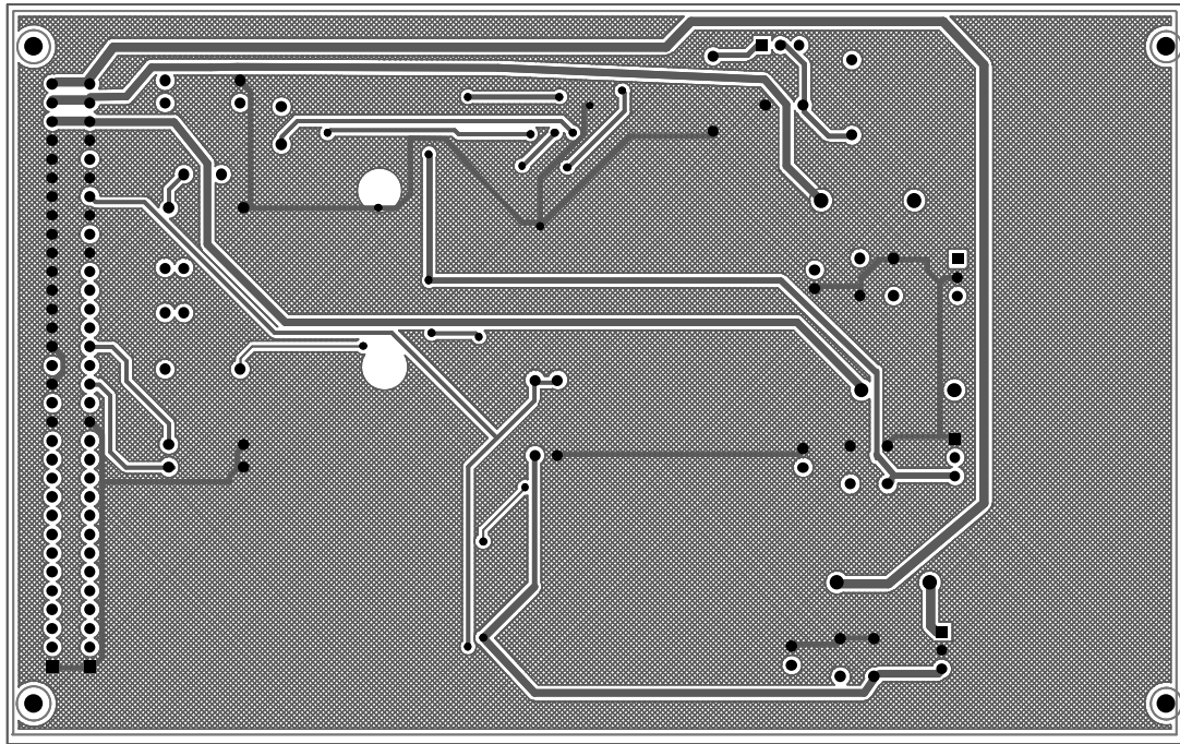
Figure: Analogue frontend module eurocard PCB (Bottom layer)
