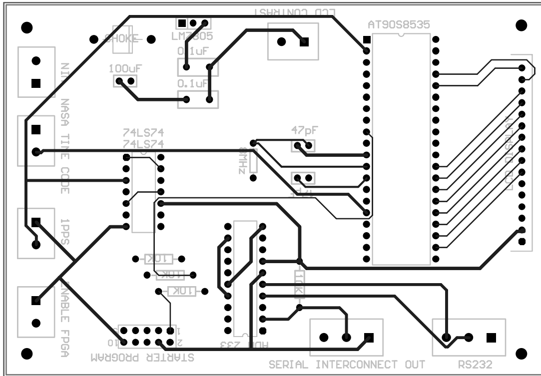
Figure: Starter module eurocard PCB (Top layer)
