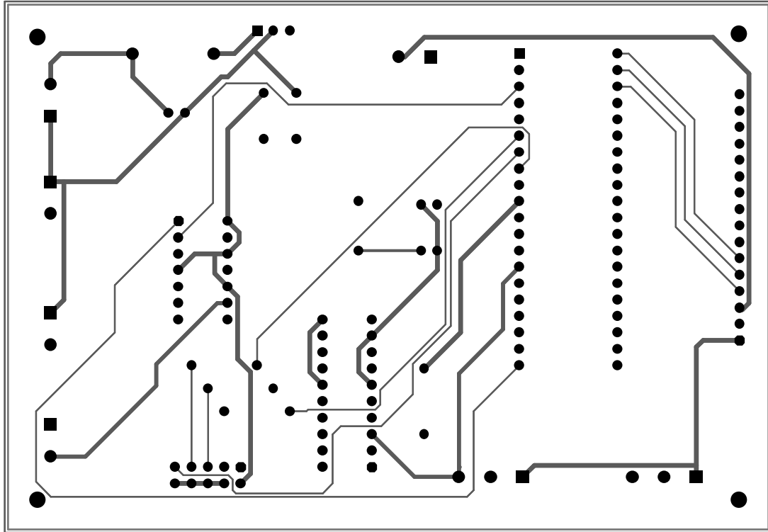
Figure: Starter module eurocard PCB (Bottom layer)
