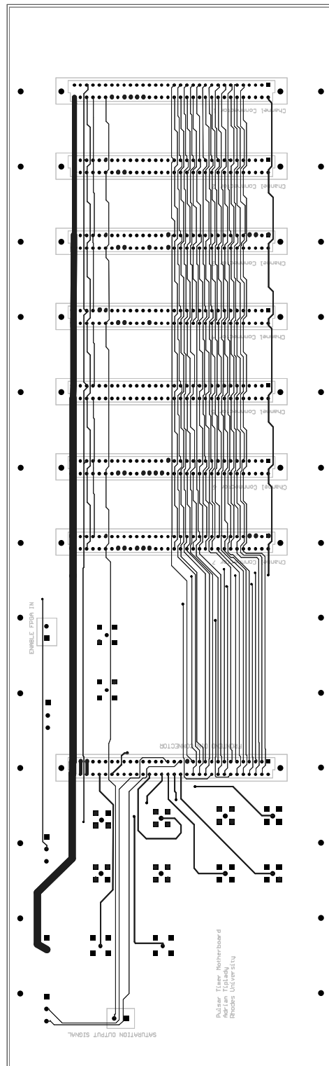
Figure: Motherboard eurocard PCB (Top layer)
