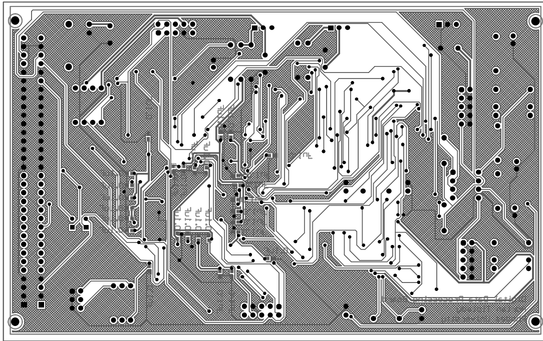
Figure: Digital backend module eurocard PCB (Bottom layer)
