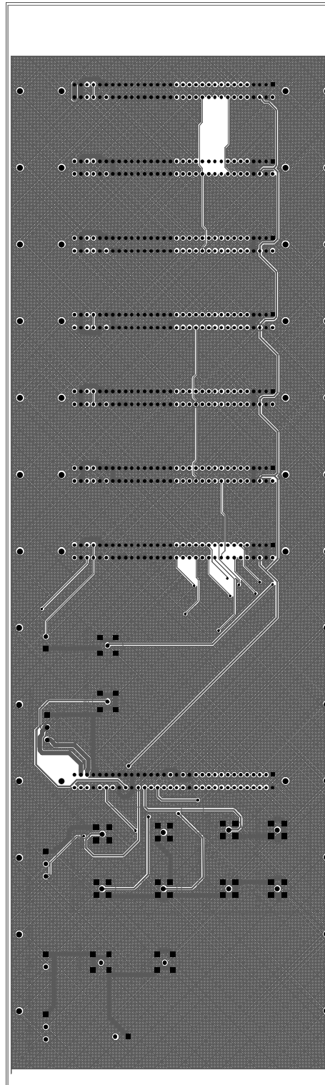
Figure: Motherboard eurocard PCB (Bottom layer)
