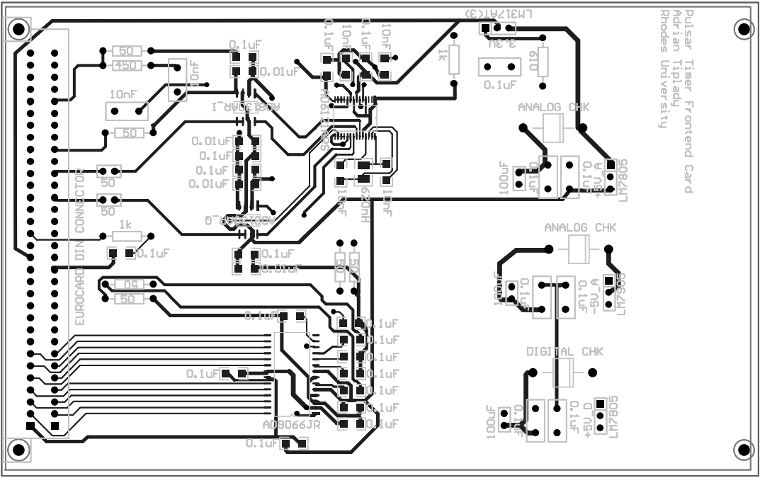
Figure: Analogue frontend module eurocard PCB (Top layer)
