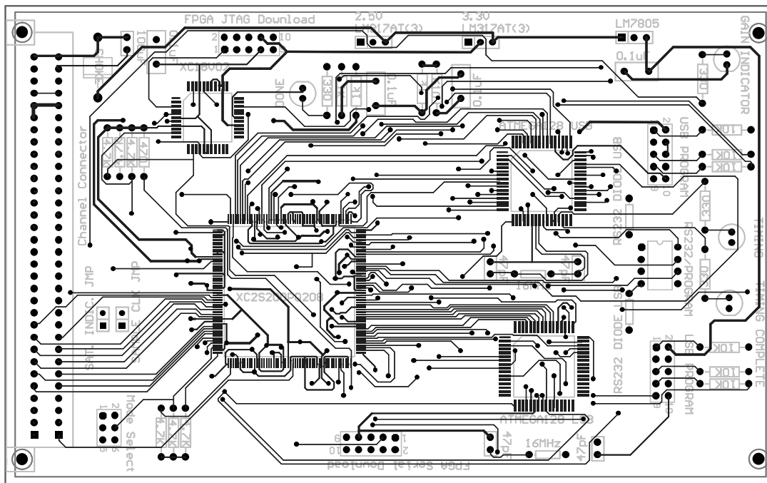
Figure: Digital backend module eurocard PCB (Top layer)
